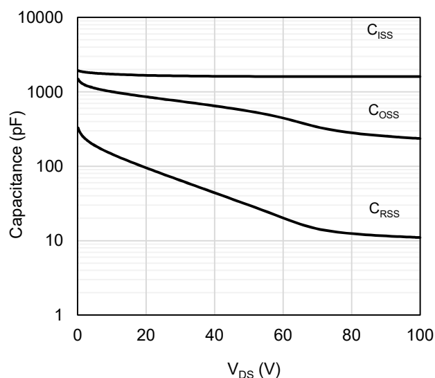
Figure 9: Capacitance Characteristics
