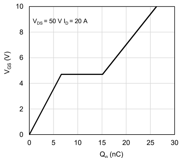
Figure 10: Gate-Charge Characteristics
