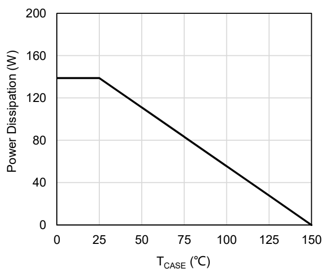
Figure 11: Power De-rating
