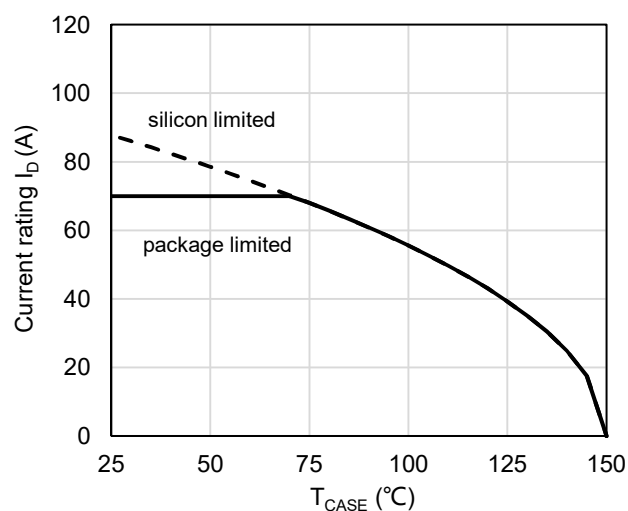
Figure 12: Current De-rating
